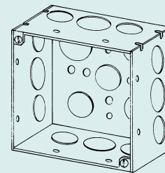
4SD-SPLRD 2⅝" Deep, Welded
