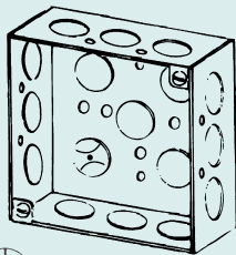
4S-1/2RD 1½" Deep, Welded
