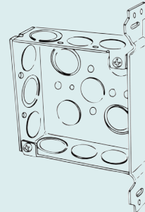
4SVB-EK-PLRD 1½" Deep, Welded Plain vertical bracket
